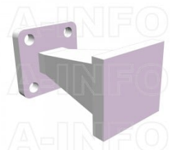
LB-28-10-ASPO Standard Gain Horn Antenna 26.5-40GHz 10dB Gain Rectangular Waveguide Interface
